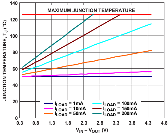
Figure 48. 100 mm 2 of PCB Copper, T_{SO1} , T_A = 50^\circ\text{C}
