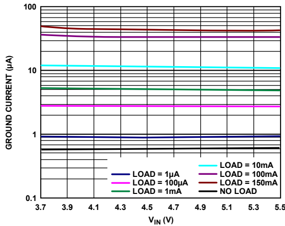
Figure 12. Ground Current vs. Input Voltage ( V_{IN} )
